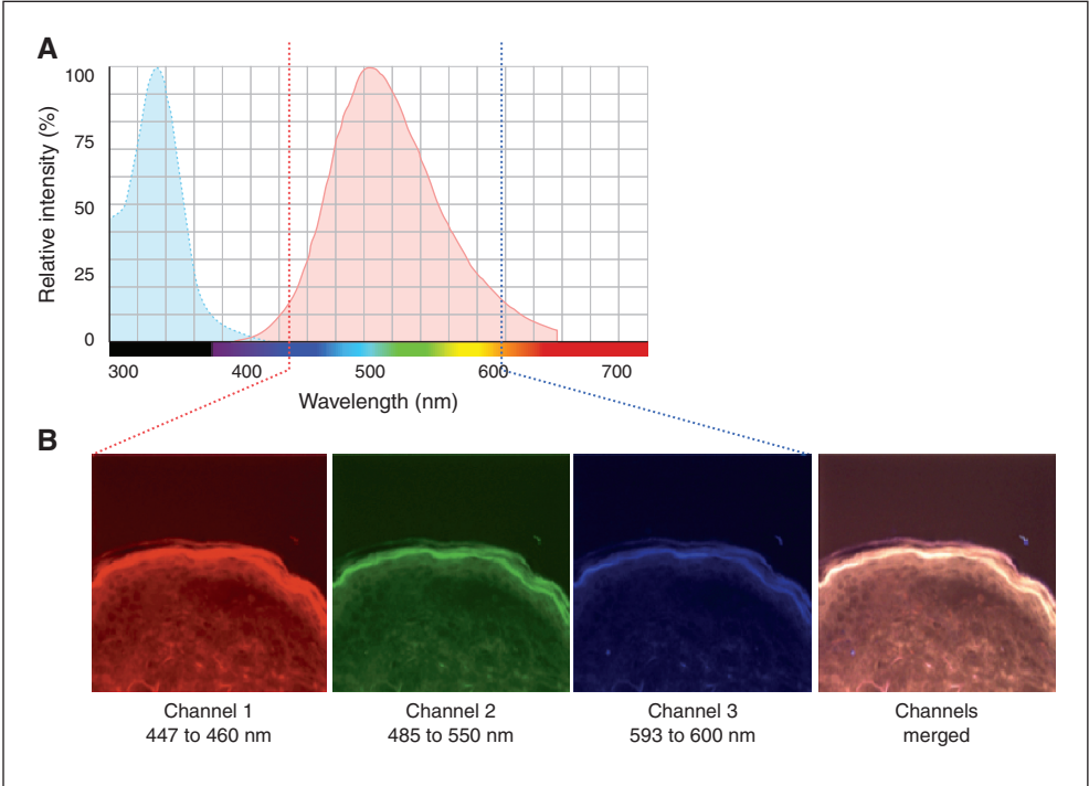
Figure 3. Imaging Mag-fura-2 fluorescence using multiphoton microscopy. A) Excitation (320 nm) and emission spectra (520 nm) of mag-fura-2, tetra potassium salt. B) We used a LaVision Biotec Nikon multiphoton system with a tunable titanium Sapphire laser to visualize the skin sections. Excitation wavelength was 740 nm and emission was detected using three non-descanned filters: 447 to 460 nm, 485 to 550 nm, and 593 to 600 nm.
